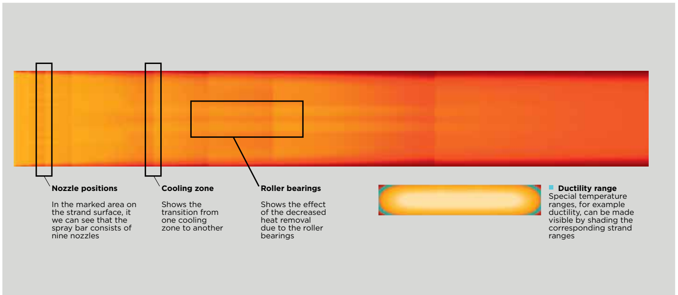
Top and cross section view of the strand in the HMI
